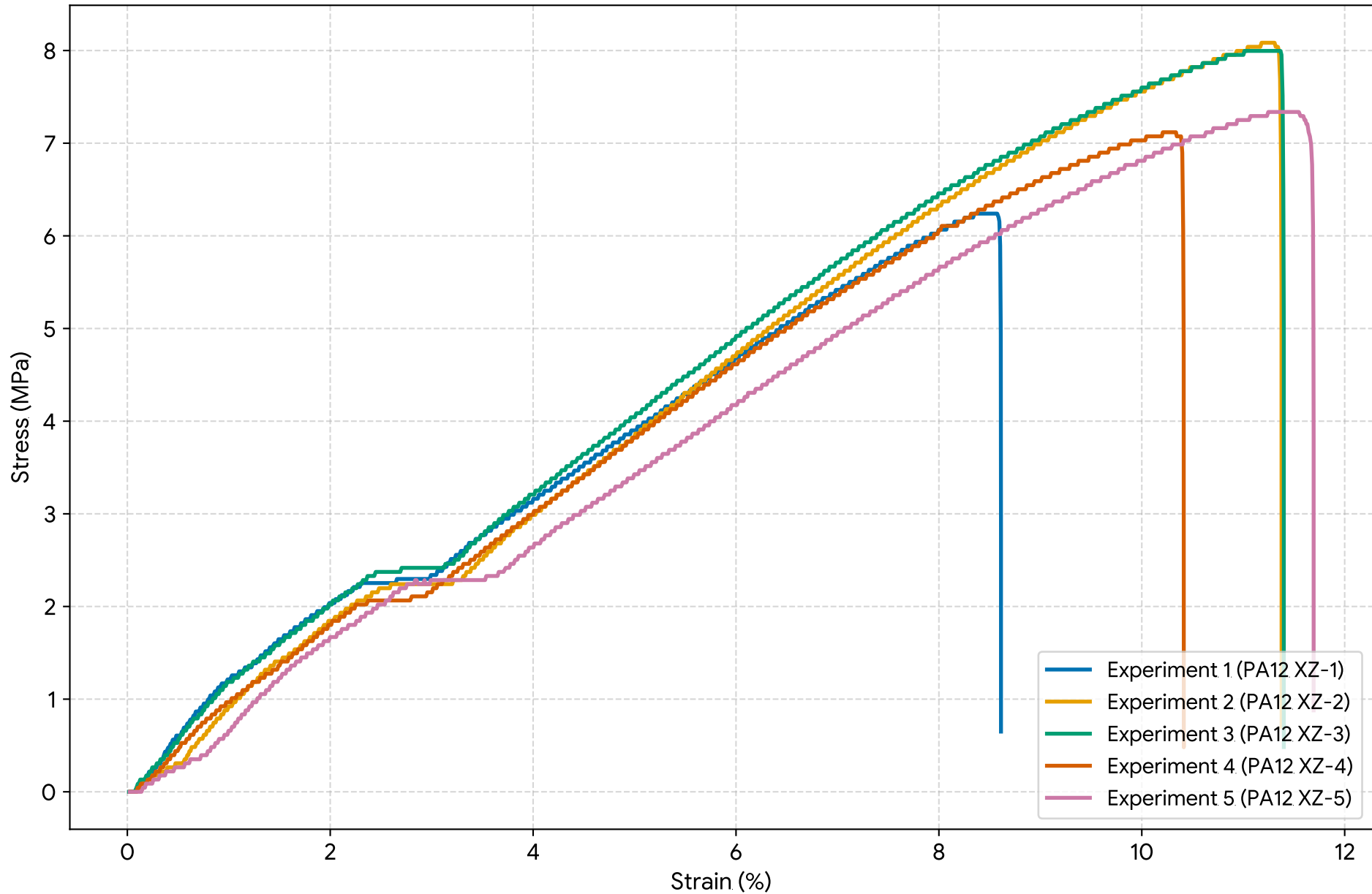
Stress-Strain Curves for PA12 XZ (5 Experiments)
